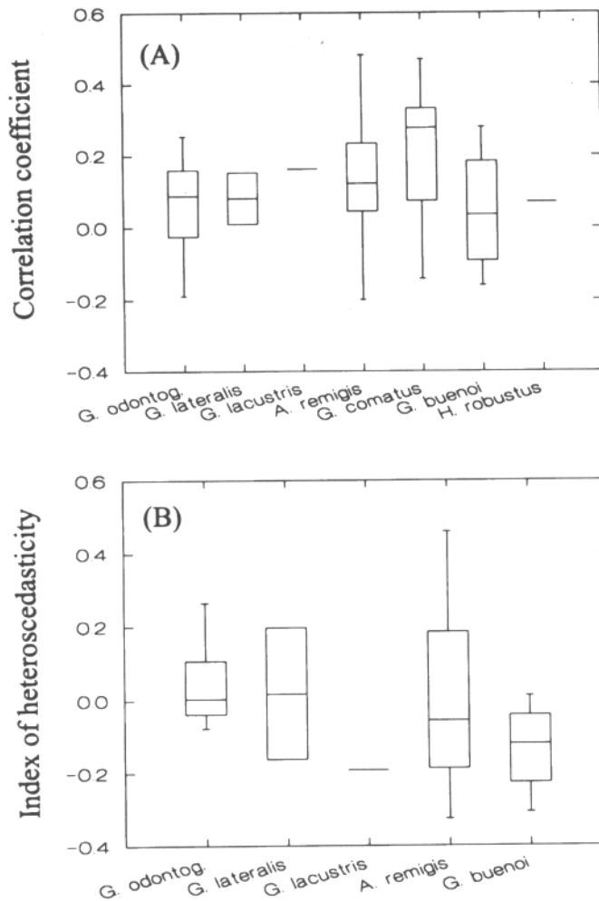
Figure 4. Box-and-whiskers plots showing interspecific variation in (a) assortative mating and (b) the index of heteroscedasticity. Boxes represent the 25th and 75th percentiles and horizontal lines within boxes represent medians.
