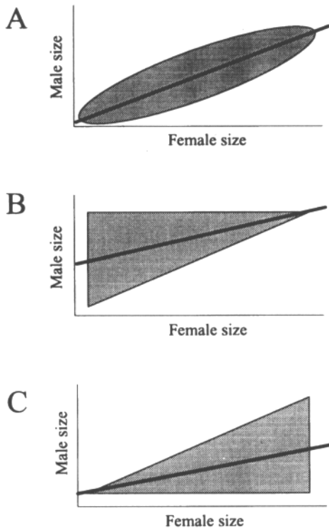
Figure 1. Three forms of assortative mating. The true form (a) is distinguished by a linear relationship between the sizes of mating males and females, where observations are distributed symmetrically around the regression line. The apparent forms (b and c) are recognized by linear relationships between male and female size where observations are delineated by a triangle around the regression line (heteroscedasticity).
