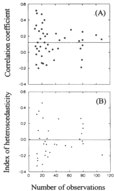
Figure 3. Plots of sample size versus effect size (i.e. funnel plots; Cooper and Hedges, 1994) for (a) the estimate of assortative mating (Pearson correlation coefficients, n = 45 ) and (b) the index of heteroscedasticity (Spearman rank correlation coefficients, n = 33 ). Solid lines represent unweighted means. Note that effect sizes tend to converge around the means with growing sample size.
