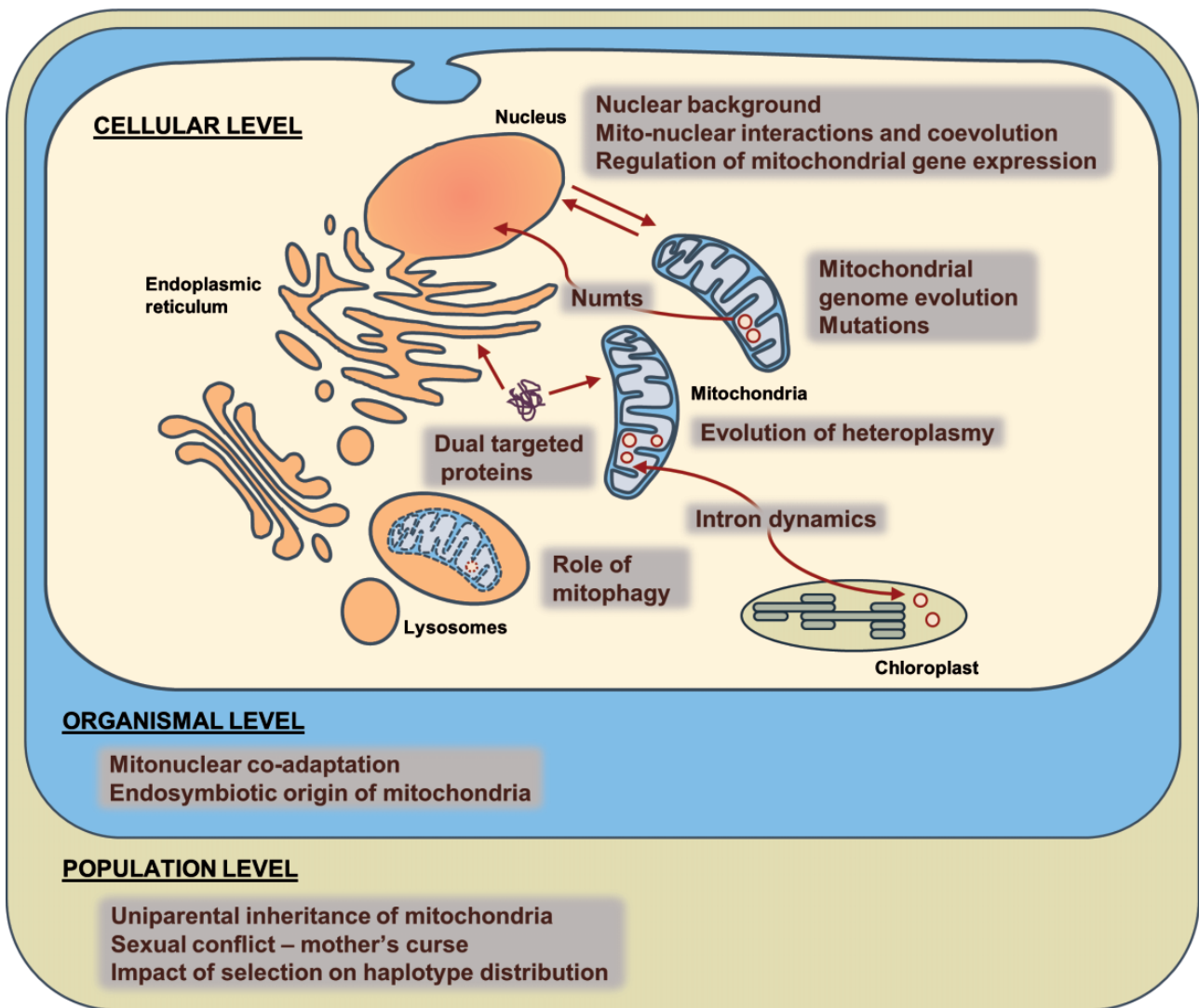
FIG. 1. —Principal topics discussed at the first Mitochondrial Genomics and Evolution satellite meeting. Topics are indicated within gray boxes.
